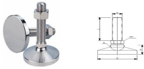
Carbon Steel Swivel Leveling Feet
